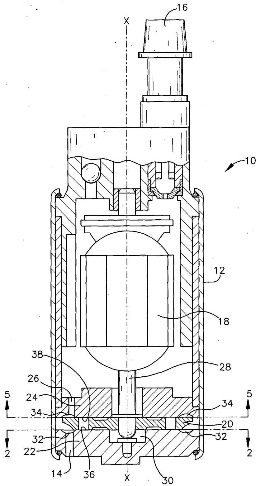
Fig.1 (PRIOR ART)
